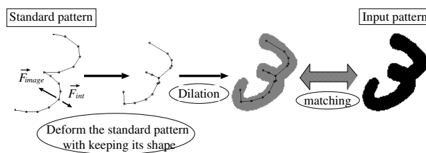
Figure 4. An illustration of matching
