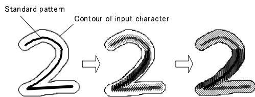
Figure 9. Dilation of the deformed standard pattern
