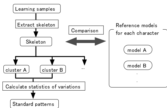
Figure 2. Procedure of learning standard patterns
