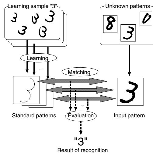
Figure 1. Overview of the recognition system
