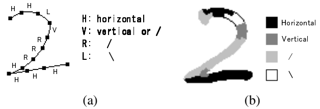
Figure 10. Orientation attributes on a standard pattern (a) and an input character (b)
