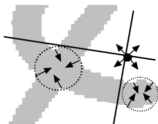
Figure 6. Orientations around the crossing point and the end point of the input character
