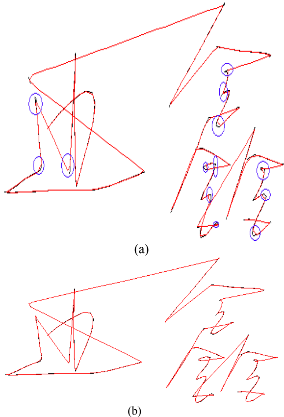
Fig.3 Preprocessing of on-line signature: (a) Re-sampling the signature uniformly with equidistant spacing. These blue circles label the lost cusps. (b) Re-sampling with our proposed algorithm. There has no lost cusp. The black tracking represents the original handwriting while the red tracking denotes the re-sampled handwriting.
