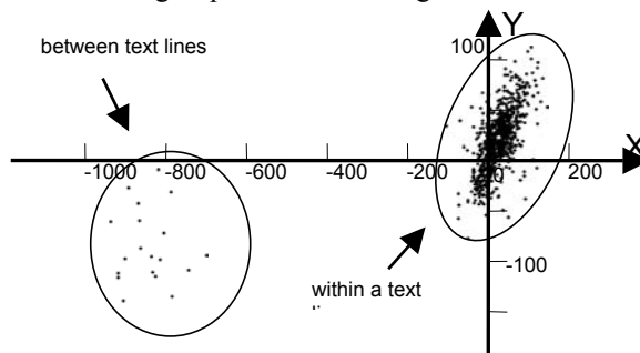
Fig. 6. Clustering of off-strokes.
