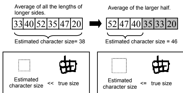
Fig. 4. Estimation of character size.
