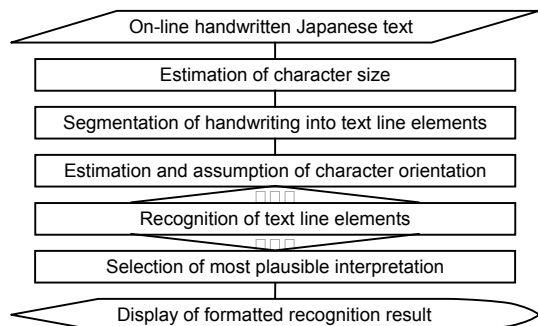
Fig. 3. Flow of processing.
